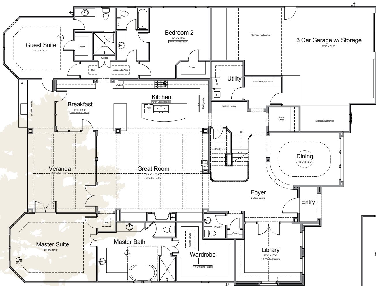
FIRST FLOOR
